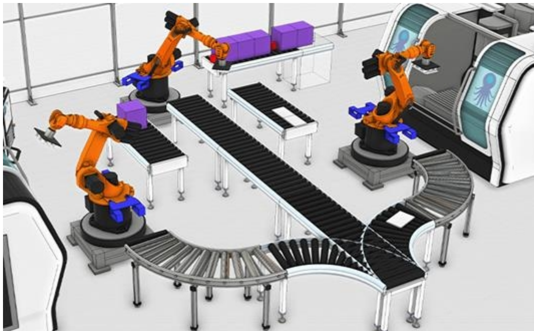
Figure 4: Octopuz OLRP - multiple robots and even CNC machines can be handled in the simulation. The software helps you calculate cycle time and other useful production statistics.
