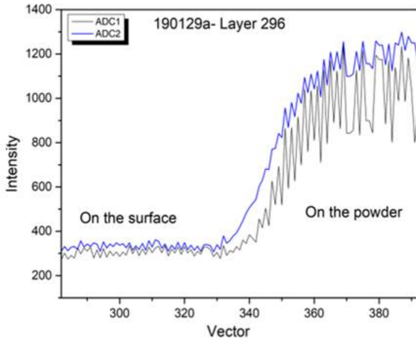
Figure 2: Example of an output file from MPM system for SLM showing the sensitivity of the signal to manufacturing conditions (scan on molten surface vs. scan on powder)
