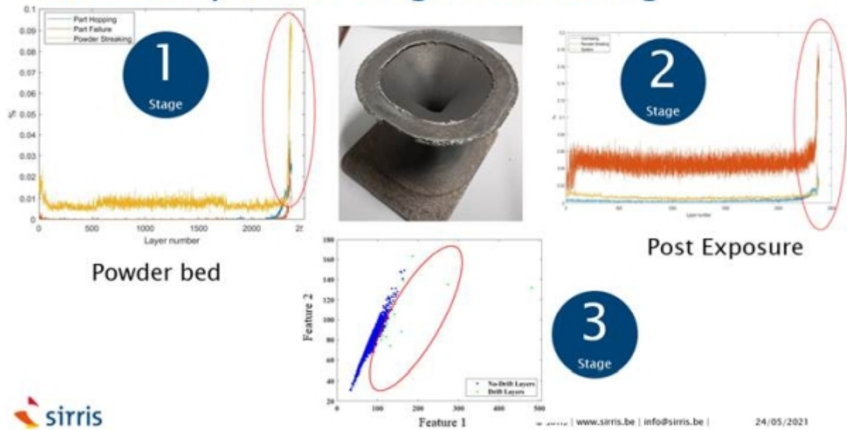
Figure 3: Automated anomaly detection using machine learning, applied in a case study on a benchmark piece
