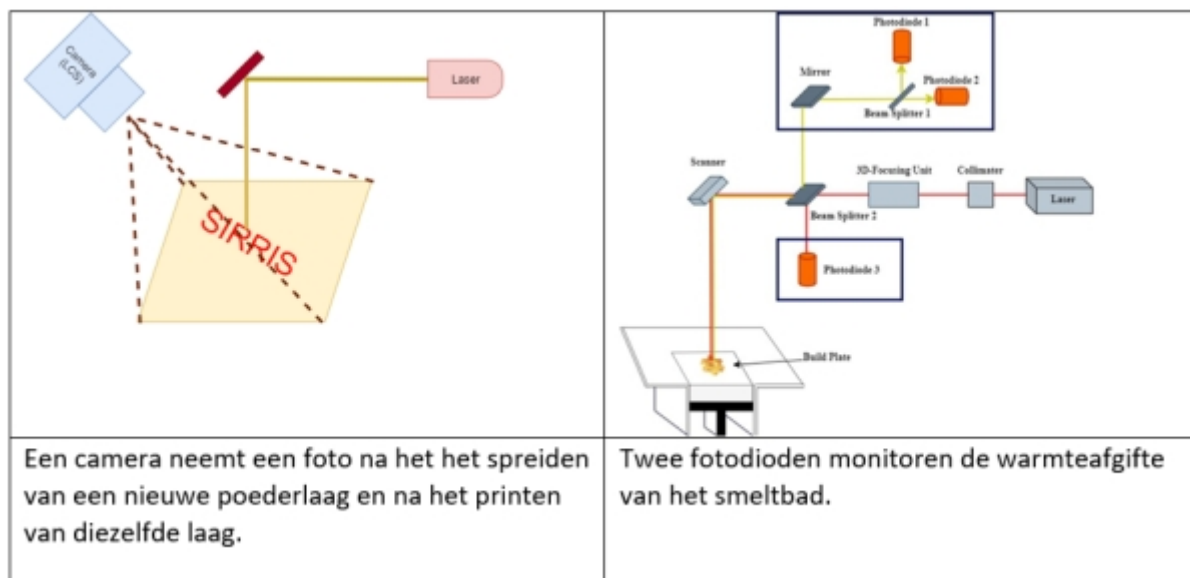
Figure 1: In-situ monitoring equipment on the LBM machine at Sirris
