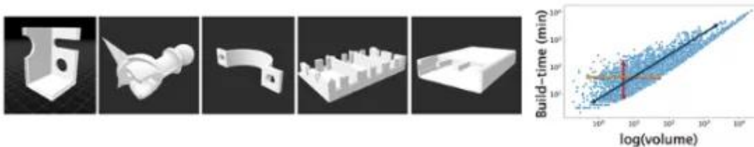
(left) Examples of the modeled 3D objects with diverse characteristics, (right) complex and non-linear relations between the objects' volumes and their build times
