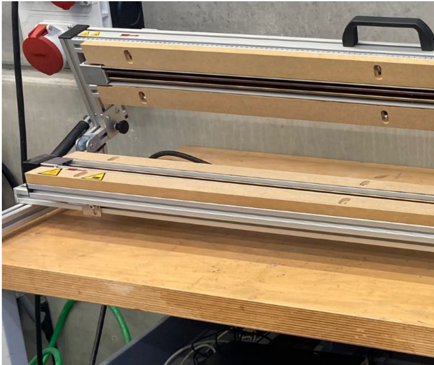
Figure 2: the bending machine that took care of the local melting of the PLA matrix, in order to be able to bend the sandwich structure afterwards.
