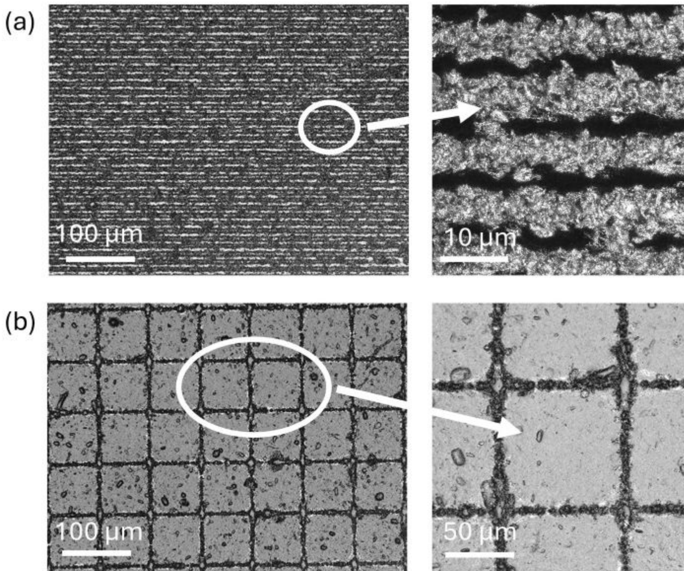
Figure 2. Laser-patterned nanocellulose coatings with (a) one-dimensional patterns, (b) two-dimensional patterns. Pattern sizes are limited by the laser spot size and can be at minimum 15 µm
