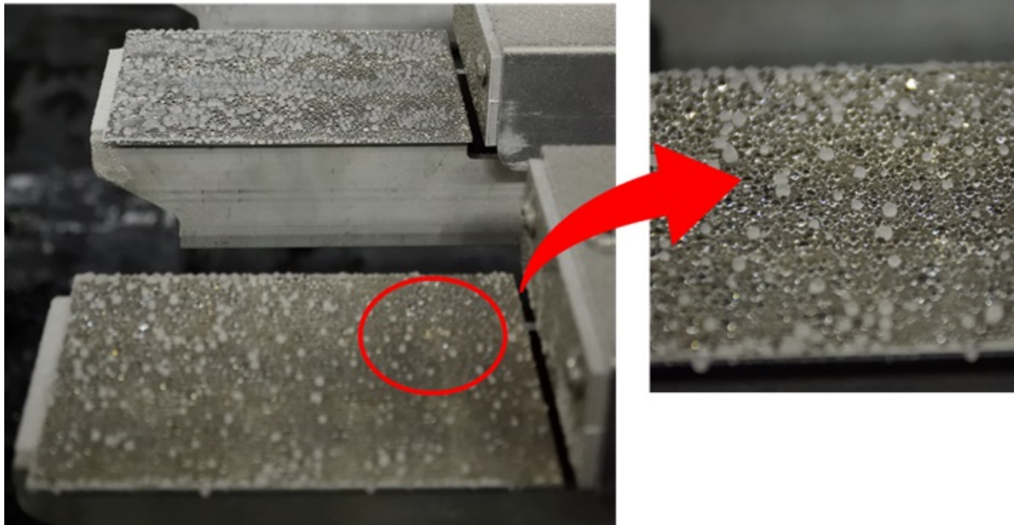
Figure 1 shows this effect: supercooled droplets at -20\text{ }^{\circ}\text{C} remain round and mobile thanks to trapped air pockets, while others already start freezing. A visual proof of delayed nucleation.
