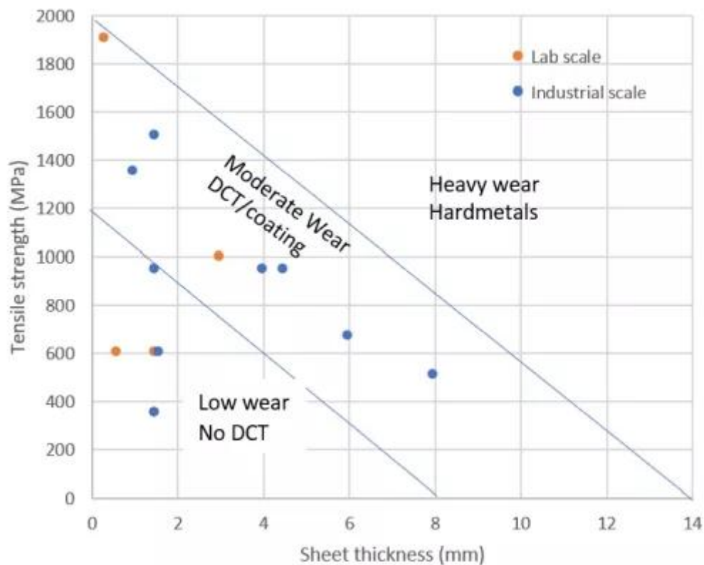
Working diagram DCT
