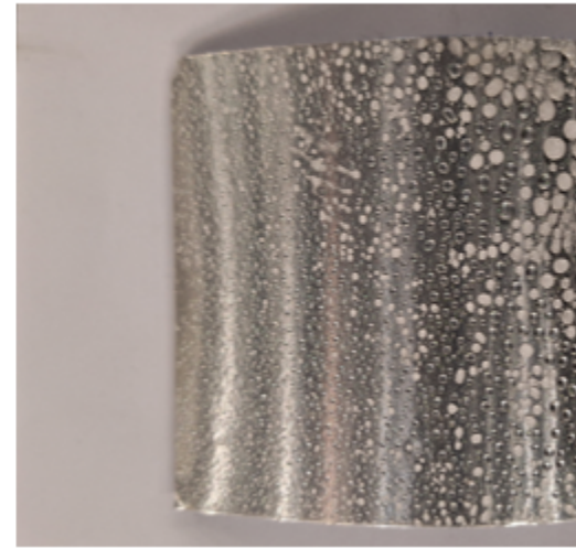
Hybrid texture 1
